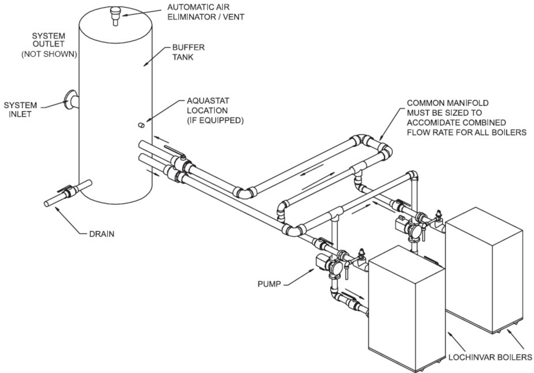
(FIG. 26) BUFFER TANK PIPING
